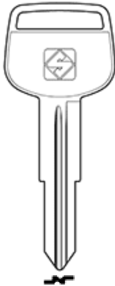
TOY42
